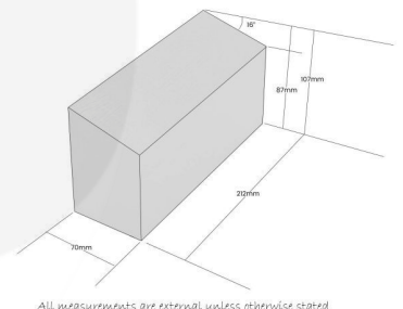
16 Degree Angled Plinth | 212x70x107
