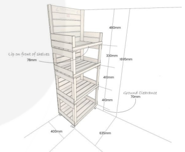
4-tier Open Crate Shelving unit | 625x400x1695
