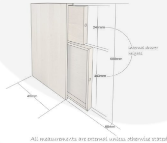
Oak Chopping Board & Tray Unit 68X411X688
