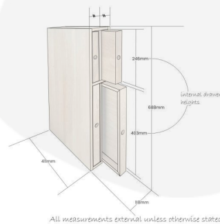
Oak double chopping board & tray unit 118x411x688
