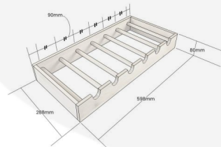
Oak 6x1 6 Bottle Wine Rack | 598x288x80
