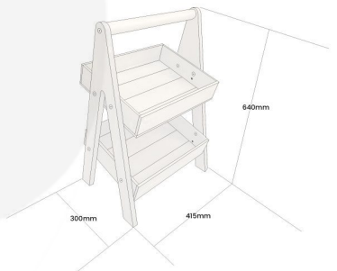
2-Tier Adjustable A-Frame | 415x300x640
