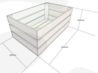
Crate 600x370x250
