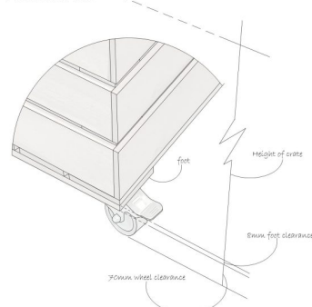
Mobile Crate Detail
