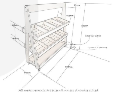
Mobile 3-Tier Slanted Merchandiser Display Stand | 1190x370x1145
