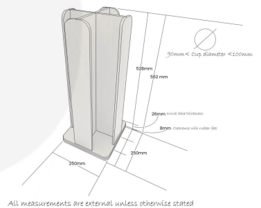
Oak 4 Compartment Rotating Cup & Lid Holder | 250x250x562
