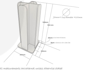
Oak 4 Compartment Rotating Cup & Lid Holder | 250x250x562
