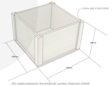
Oak Condiment Holder 4-Sided Table Talker | 178x178x116
