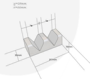
Redwood 2 Taco Stand | 207x95x70
