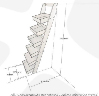
6-tier Slanted Tray Wall Ladder Display Stand 411x536x1607
