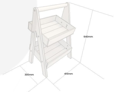
2-Tier Adjustable A-Frame | 415x300x640
